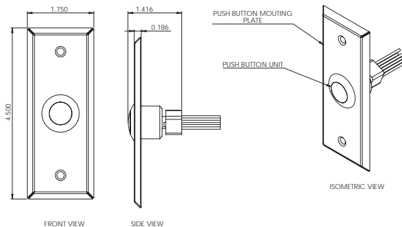
Push to exit buttons (Narrow and Wide)
