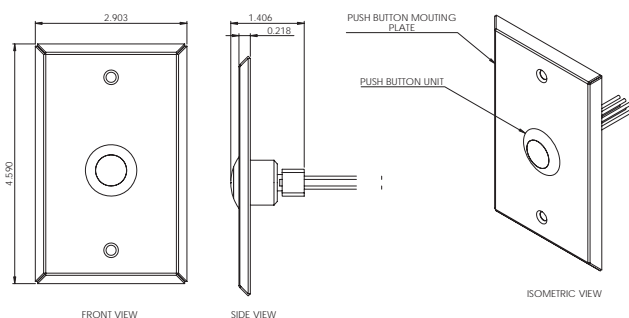
Push to exit buttons (Narrow and Wide)
